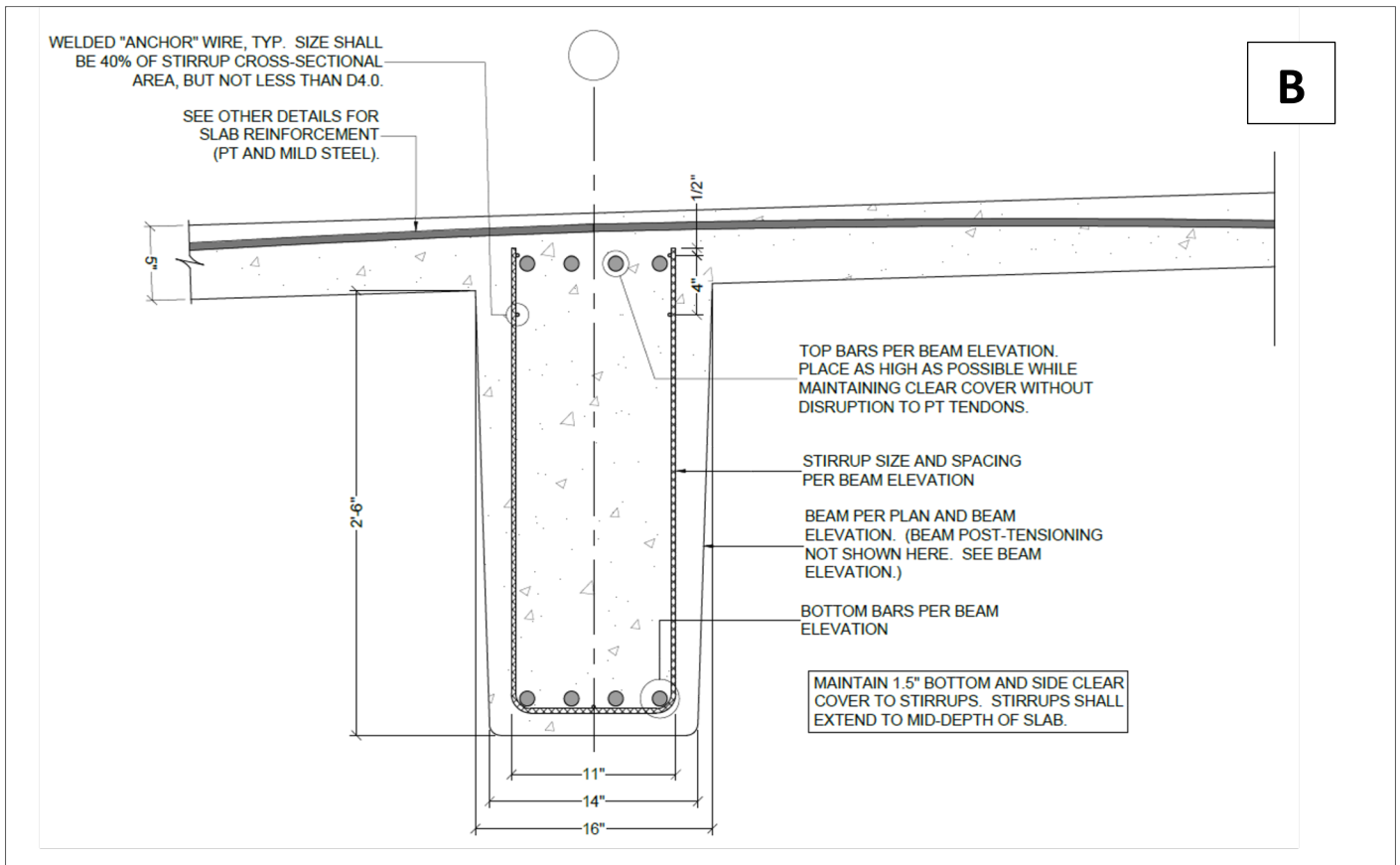
Figure 3.3: The engineer's contract drawings provide a WWR-specific section showing the U-stirrup with welded intersection curtailment in the compression zone. Sufficient structural geometry is furnished for the WWR detailer to derive the stirrup geometry itself.
